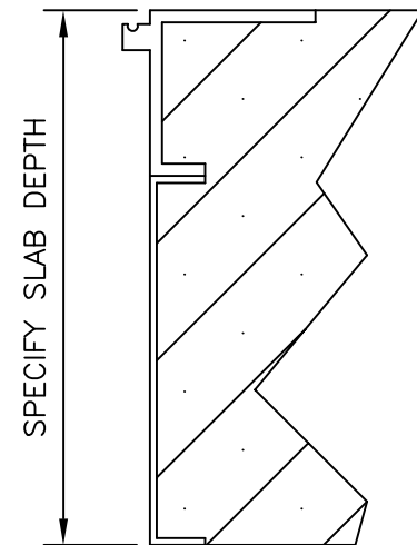
SLAB SKIRTING
