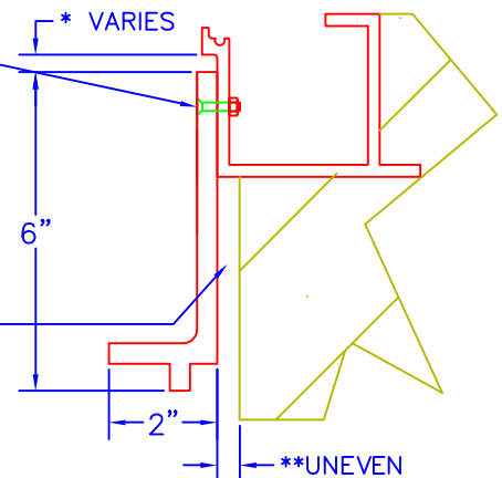
CHANNEL FRAME
